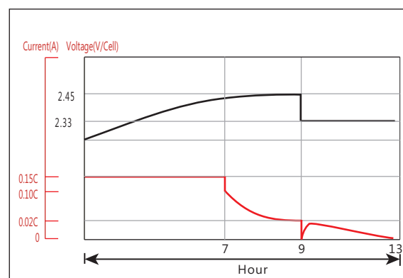
Charge performance
