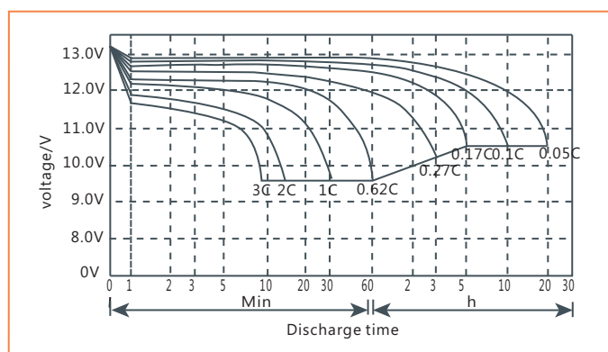
Discharge performance
